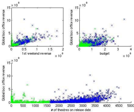
Figure 3: Training data after K-means clustering
