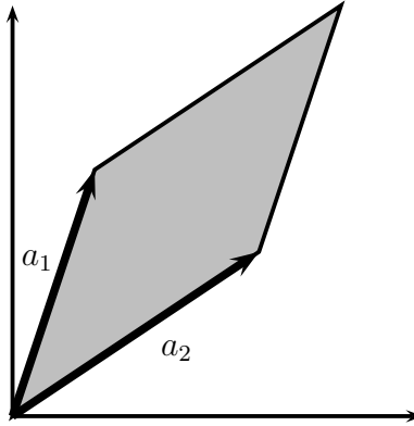
Figure 1: Illustration of the determinant for a 2 \times 2 matrix. Here, a_1^T, a_2^T \in \mathbb{R}^2 are the rows of some 2 \times 2 matrix A , and set S corresponds to the shaded region (i.e., the parallelogram). The absolute value of the determinant, |A| , is the area of the parallelogram.
