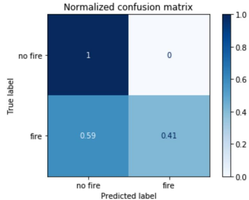
Figure 3. Confusion Matrix of SVM results
