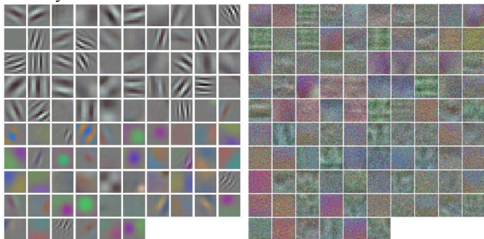
Figure 4 Nicely converged 1st layer weights (left) vs noisy weights (right)
