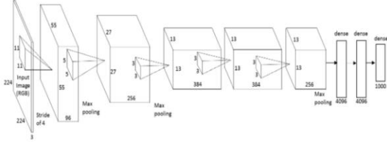
Figure 2 CaffeNet architecture
