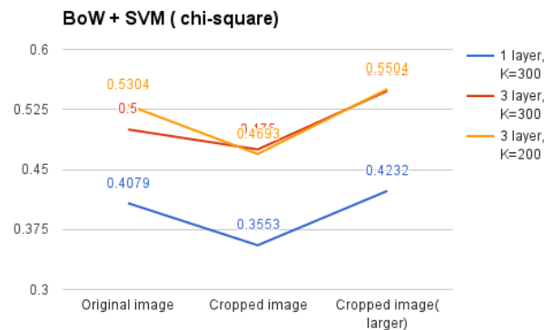
Figure 8 Plot of our results
