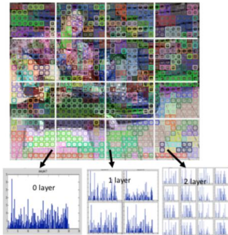
Figure 7 BoW features
