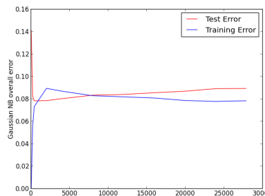
(a) Gaussian NB training vs. test errors
