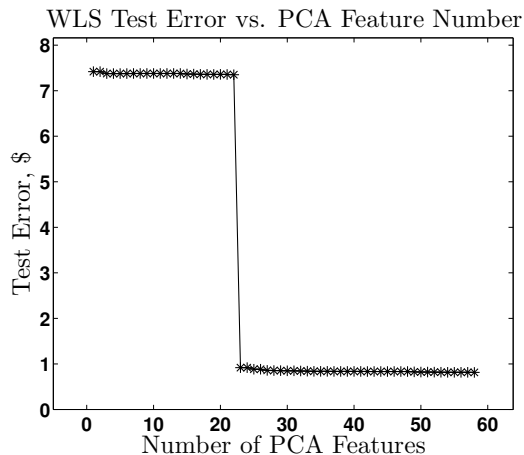
Figure 2: WLS WEPS versus PCA Feature Number.
