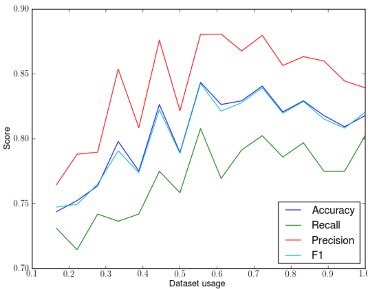
Scores with dataset usage, testing with constitution/puns
