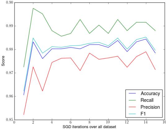
Scores with SGD iterations K
