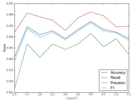
Scores with overfitting parameter C
