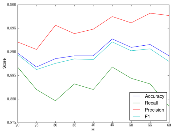
Scores with number of hidden variables H
