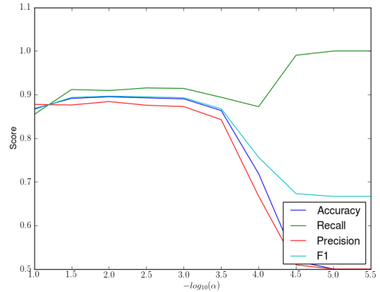
Scores with gradient descent step size \alpha
