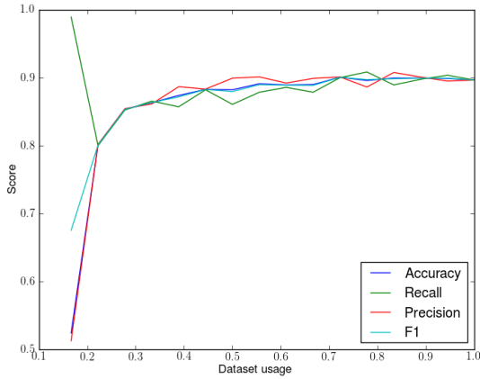
Scores with dataset utilization
